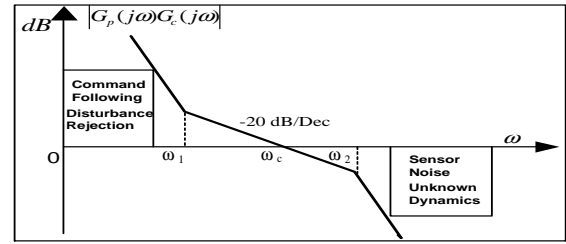
Figure 3.1 Loop-shaping
